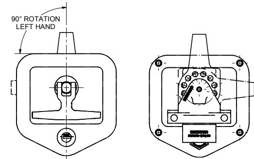
LEFT HAND ASSEMBLY
