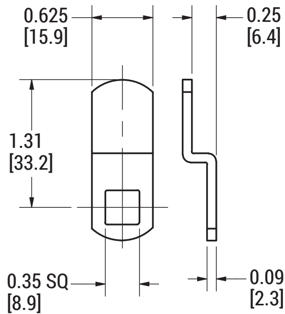
1.313" x .25" Offset Cam
