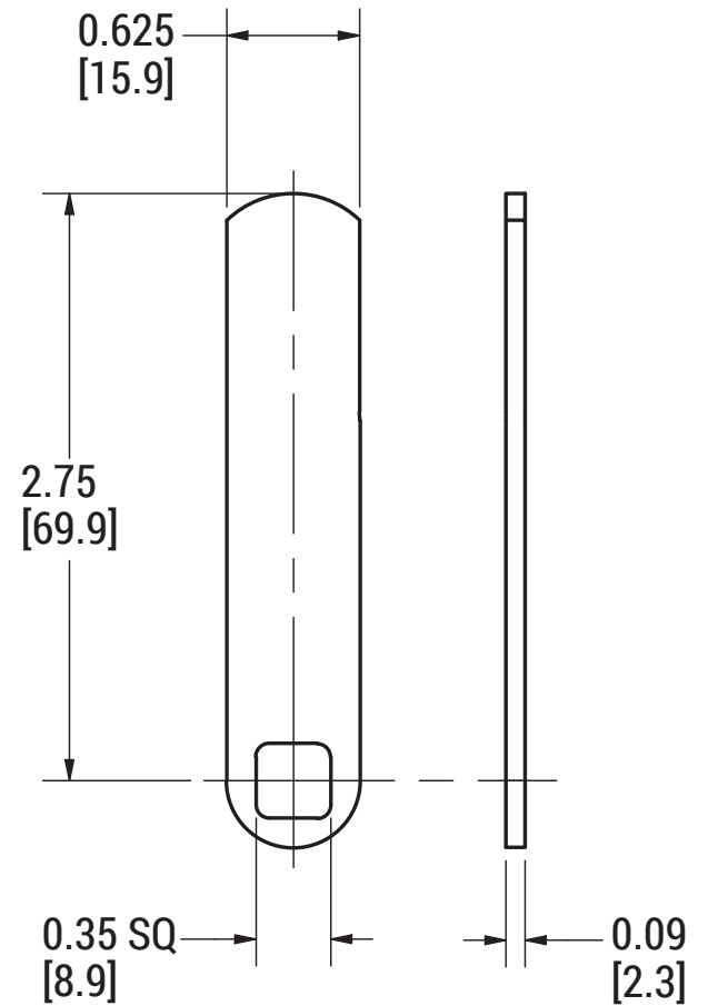
2.75" Straight Cam
