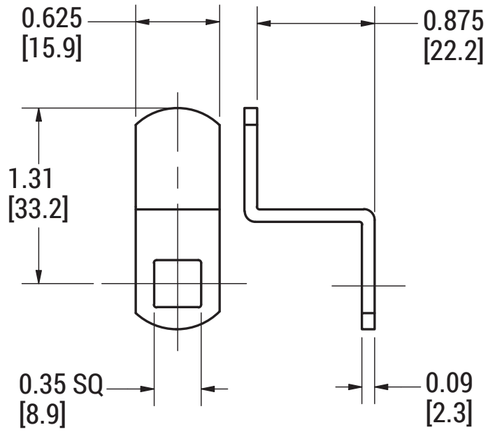
1.313" x .875" Offset Cam
